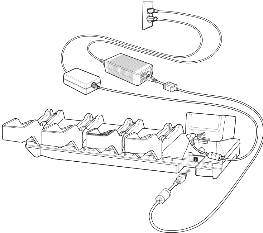
Figure 2-23 4-Slot Charge Only Cradle with Battery Charger Setup
