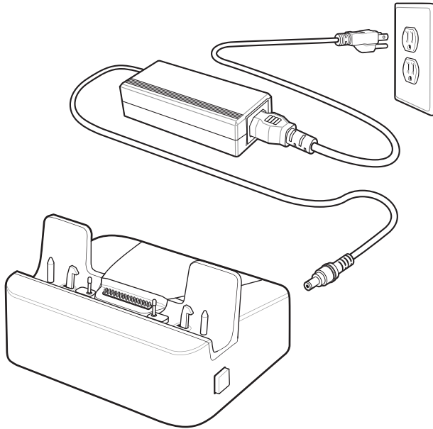
Figure 2-14 Rugged Communication and Charging Cradle - Setup
