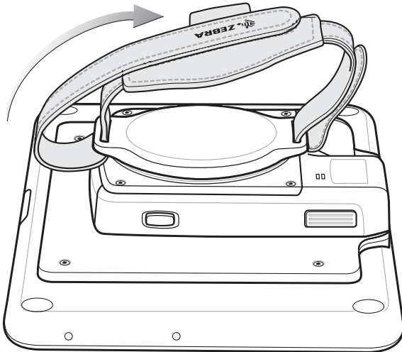
Figure 2-46 Secure Strap
