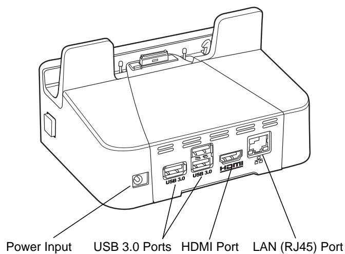
Figure 2-7 Communication and Charging Cradle - Rear View
