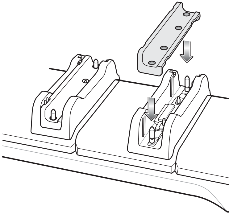
Figure 2-18 Install Insert in Slot
