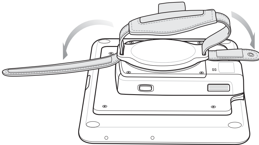
Figure 2-40 Open Straps
