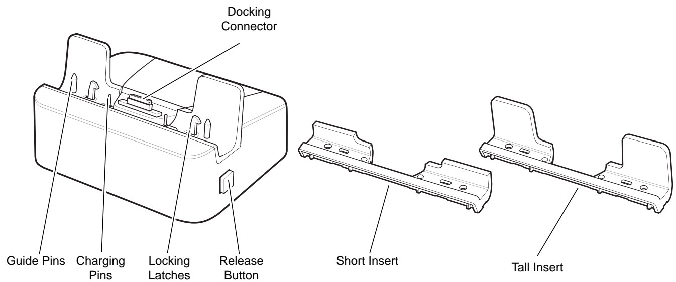
Figure 2-6 Communication and Charging Cradle - Front View
