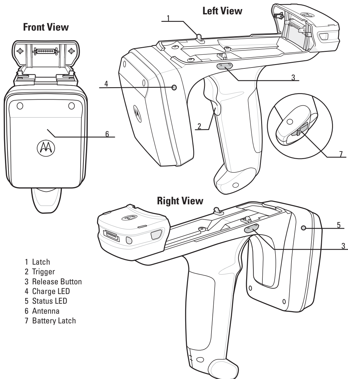
Figure 1-2 RFD5500 RFID Sled Features
