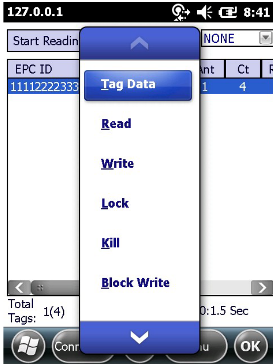
Figure 3-15 Tag Context Menu
