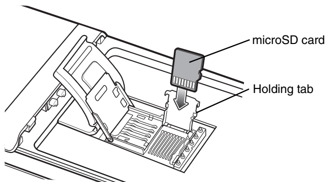
Figure 2-3 Insert microSD Card in Holder
