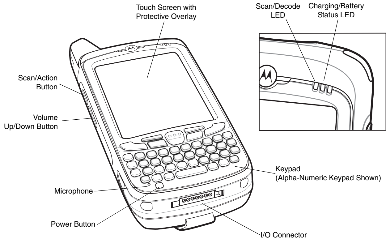
Figure 1-8 Sample of MCxx Front View
