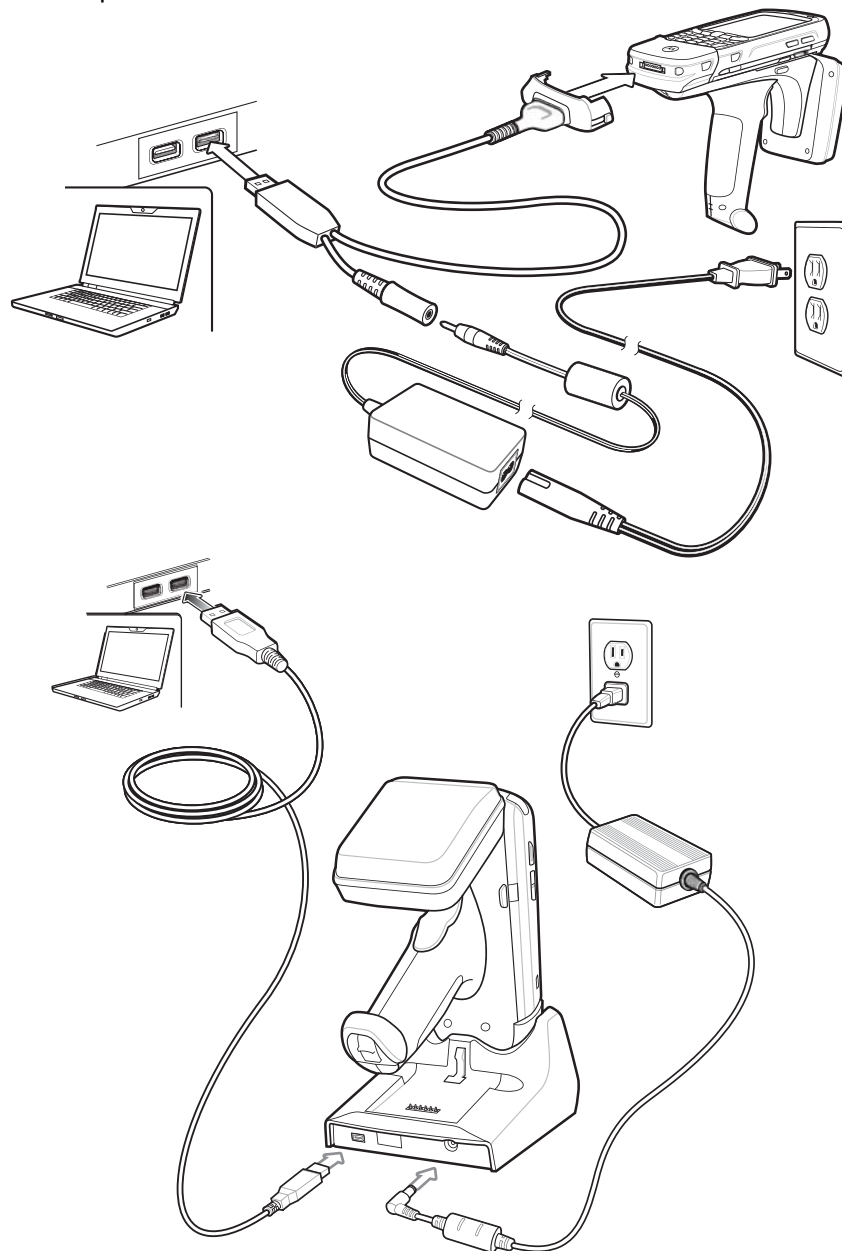
Figure 1-7 Charging and Communication
