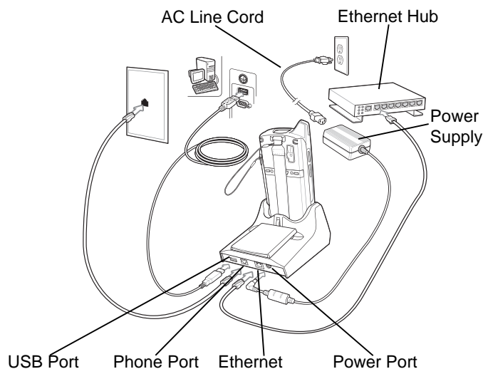
Figure 5-3 Connection Setup
