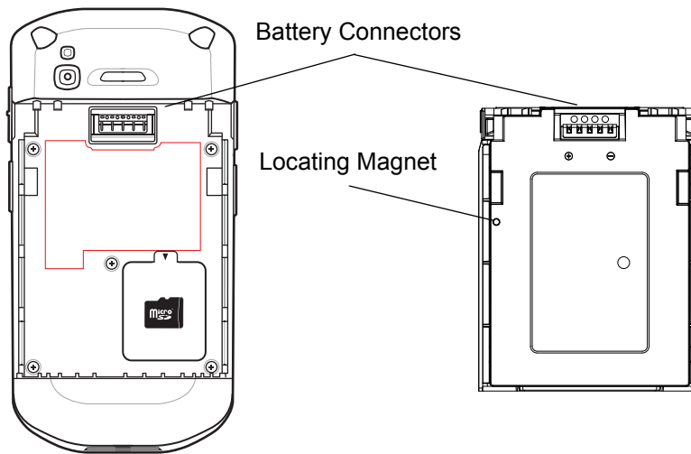
Figure 122 Battery Connectors and Locating Magnet
