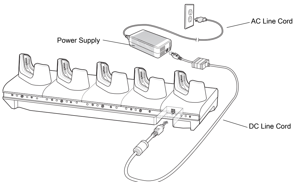
Figure 19 5-Slot Charge Only Cradle Setup
