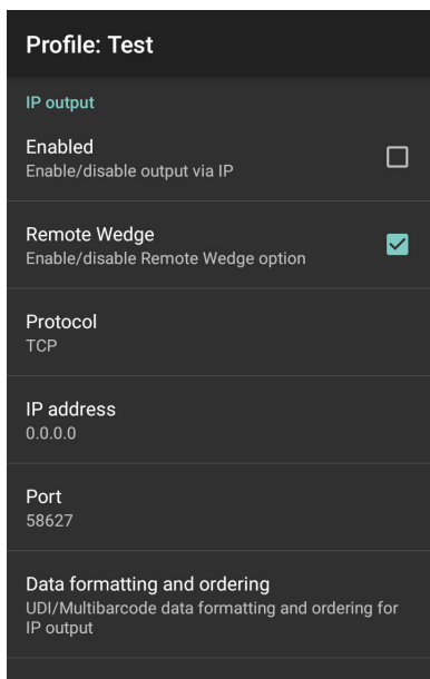
Figure 70 IP Output Screen
