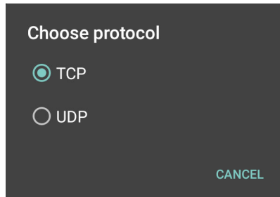
Figure 74 Protocol Selection
