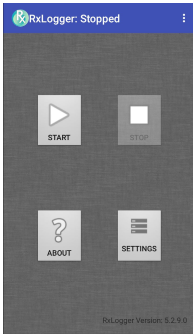
Figure 96 RxLogger
