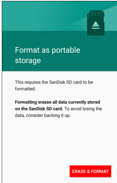
Figure 116 Format Screen
