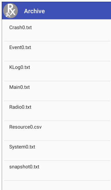
Figure 101 Archive
