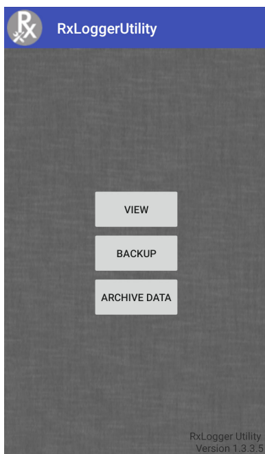
Figure 98 App View
