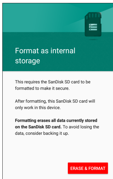
Figure 118 Format Screen
