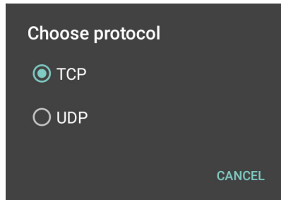
Figure 71 Protocol Selection
