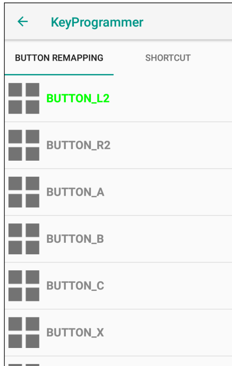
Figure 95 KeyProgrammer Screen
