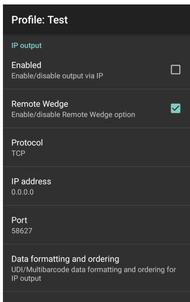
Figure 83 IP Output Screen
