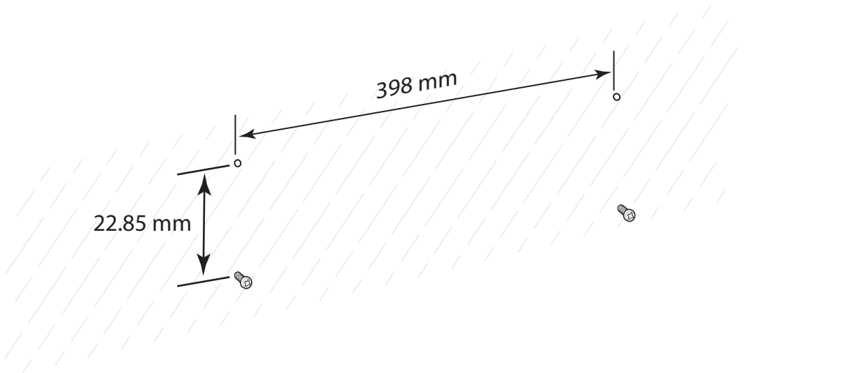
Figure 68 Horizontal Mounting Template
