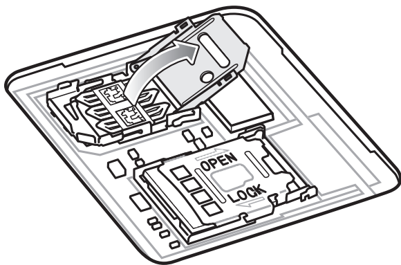
Figure 22 Lift the SIM Card Door
