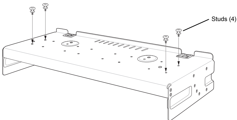
Figure 52 Install Studs
