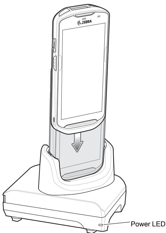
Figure 26 Battery Charging
