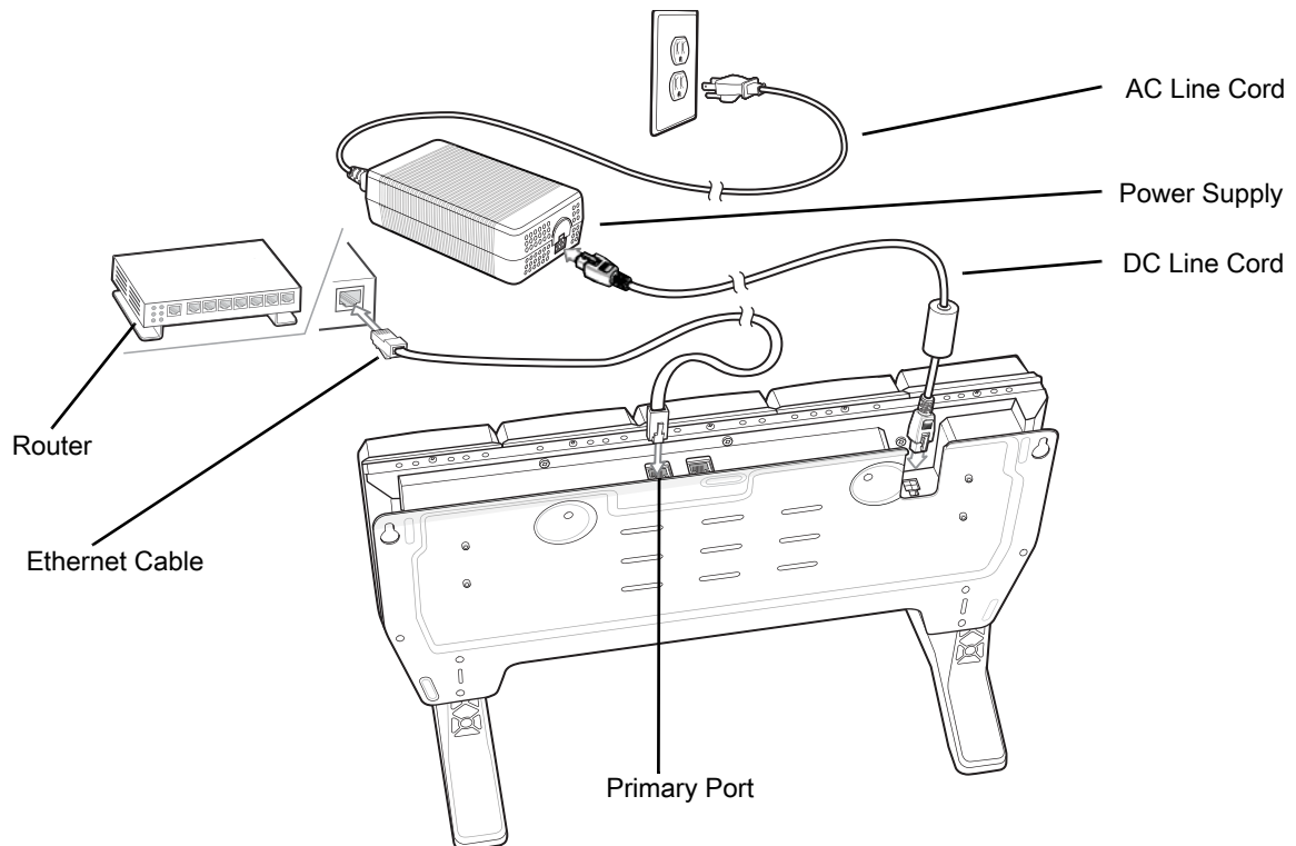
Figure 23 5-Slot Ethernet Cradle with Battery Charger Setup (Shown on Optional Desk Mount)
