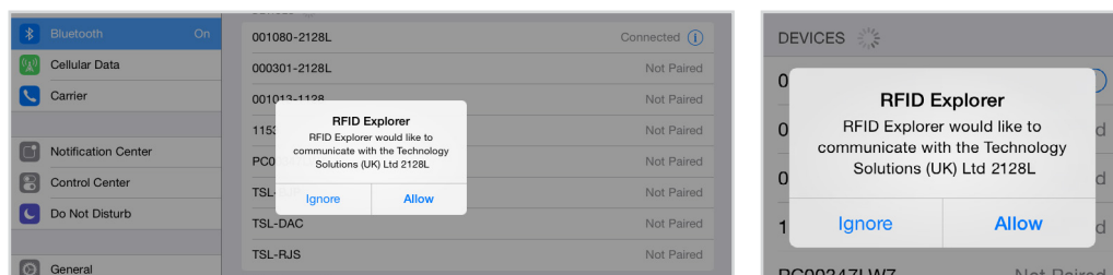
Figure 15: Allow connection
