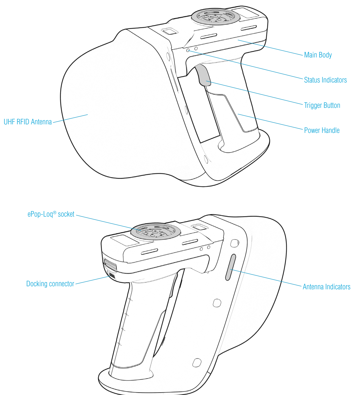
Figure 1: 2128L Reader with UHF RFID Antenna and Power Handle
