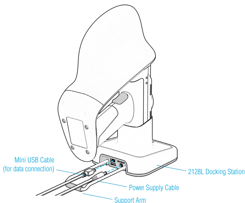
Figure 4: Charging the 2128L UHF Reader
