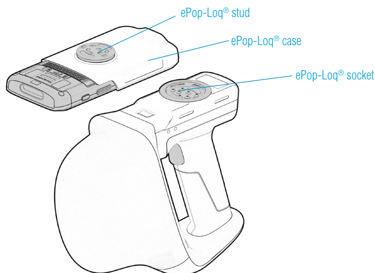
Figure 2: ePop-Loq® component parts
