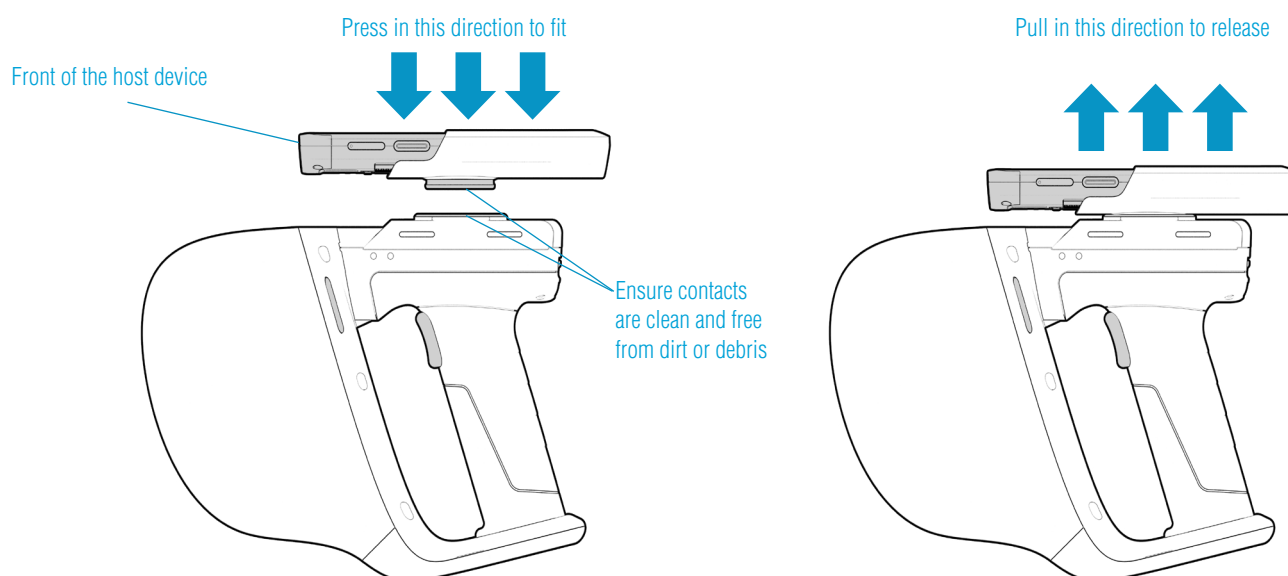
Figure 3: Attaching/Detaching an ePop-Loq® case
