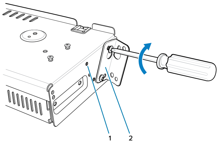
Figure 17 Flange 25° Position (4-Slot Battery Chargers)
