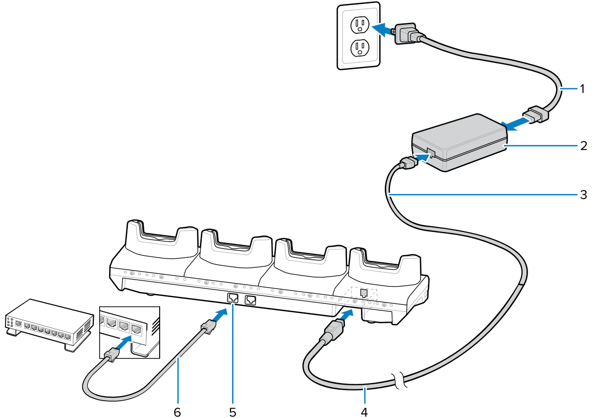
Figure 14 4-Slot Ethernet Cradle Setup
