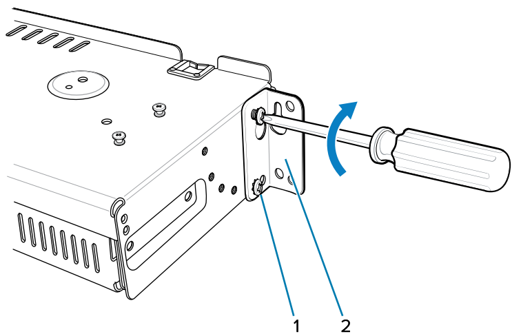
Figure 16 Flange Horizontal Position (4-Slot Cradles)
