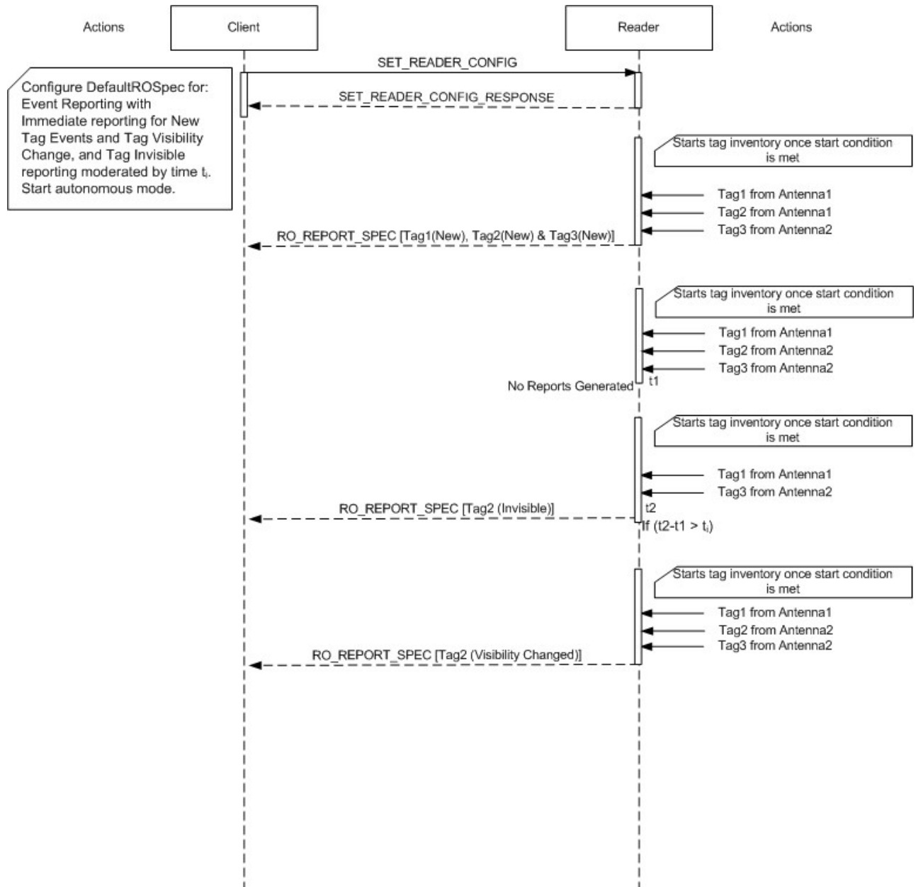
Figure 2-2 Autonomous Event Driven Reader Operation Model
