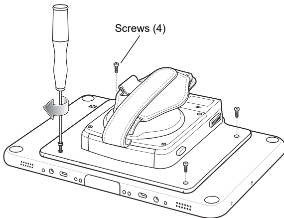
Figure 51 Secure Screws
