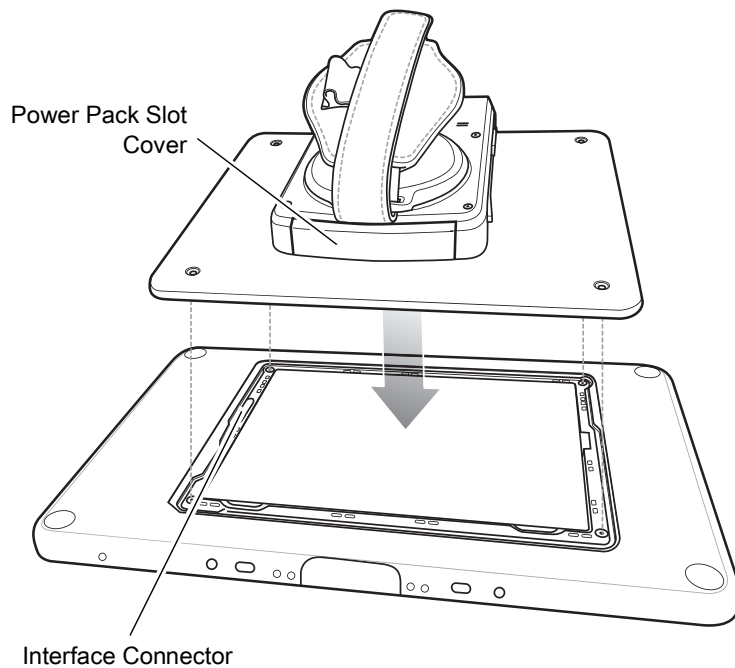
Figure 50 Align Expansion Back with 8" Configuration
