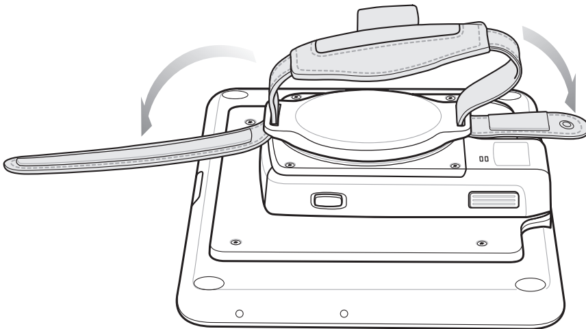
Figure 52 Open Straps
