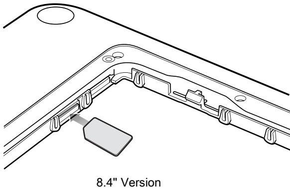
Figure 5 Inserting the nano SIM Card
