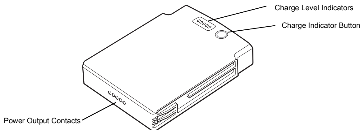
Figure 36 Power Pack
