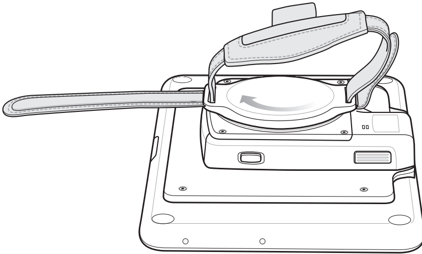
Figure 57 Feed Strap
