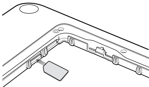
Figure 8 Inserting the nano SIM Card
