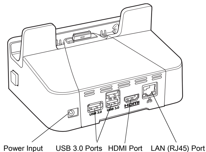
Figure 87 Communication and Charging Cradle - Rear View
