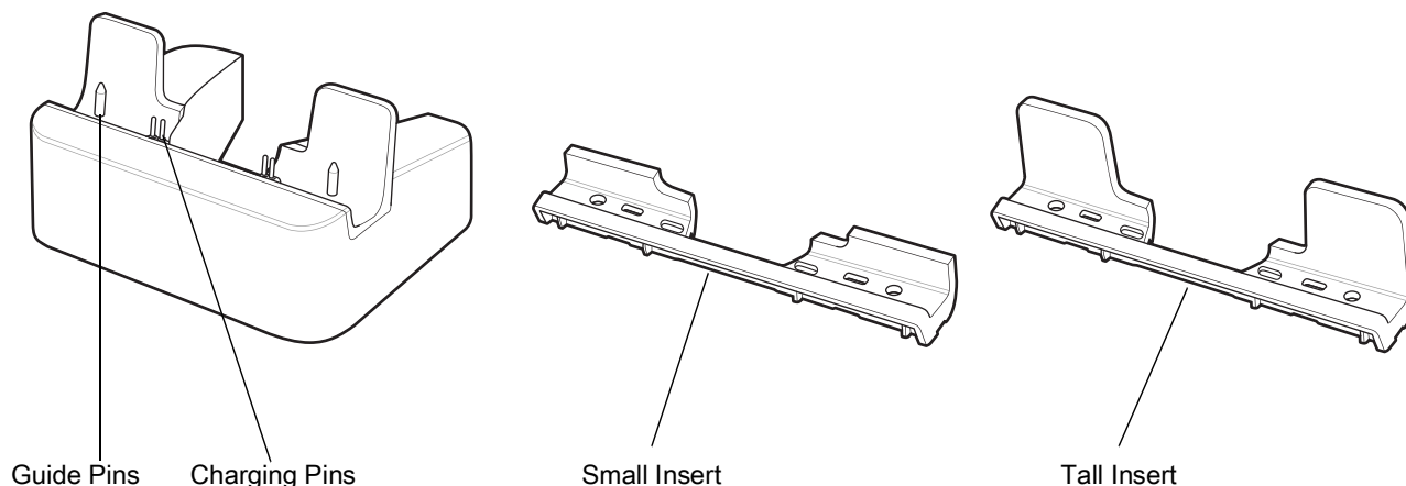
Figure 82 Charge Only Cradle - Rear View
