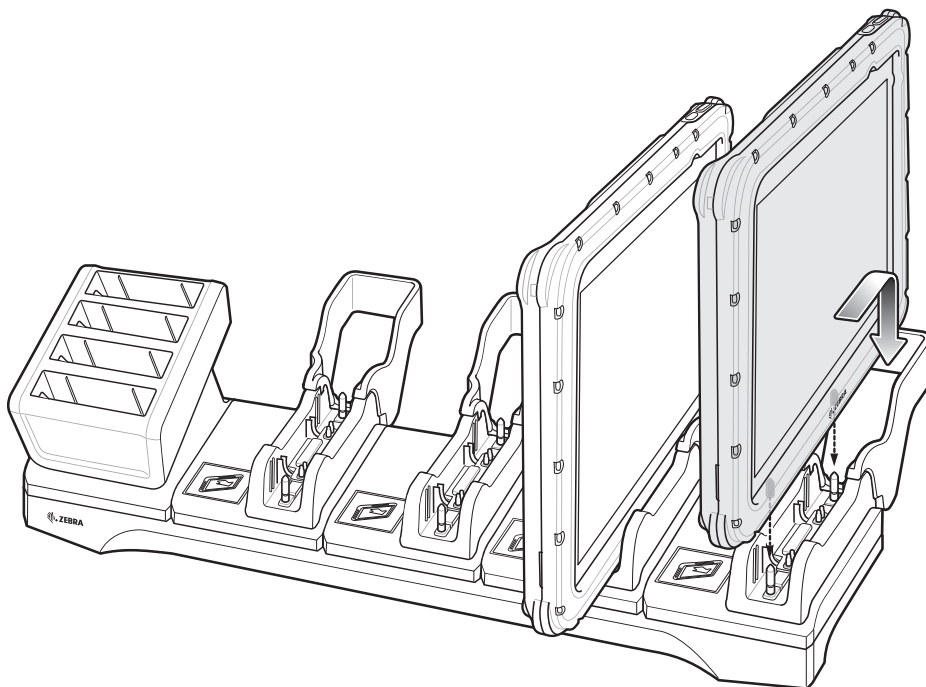
Figure 101 Insert device with Rugged Frame into Slot
