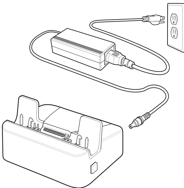
Figure 94 Rugged Communication and Charging Cradle - Setup
