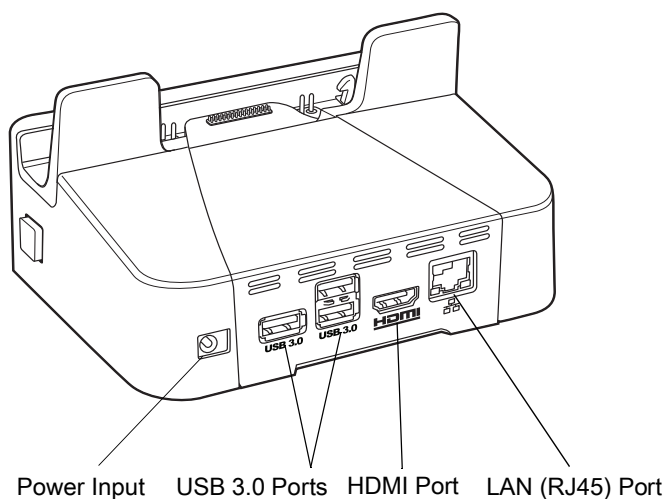
Figure 93 Rugged Communication and Charging Cradle - Rear View
