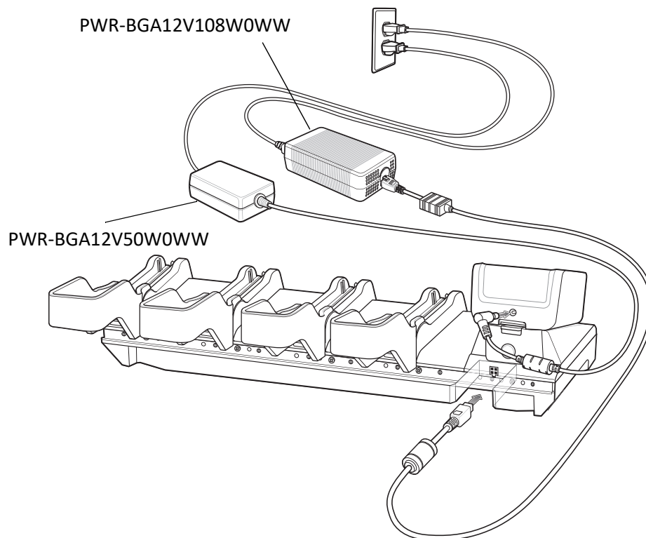
Figure 99 Power Setup with Optional Charger
