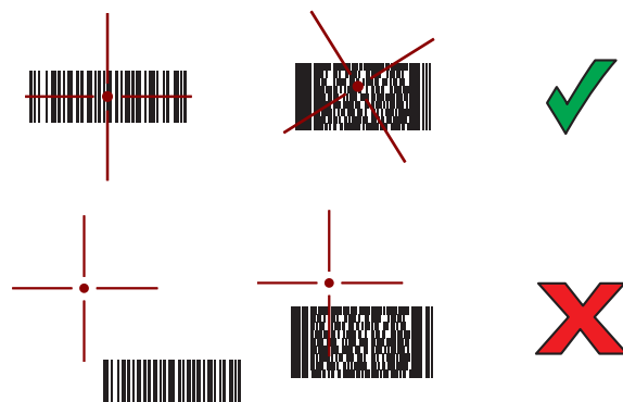
Figure 60 SE4750 Expansion Back Aiming Pattern
