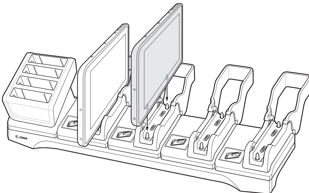
Figure 100 Insert ET5X without Rugged Frame into Slot
