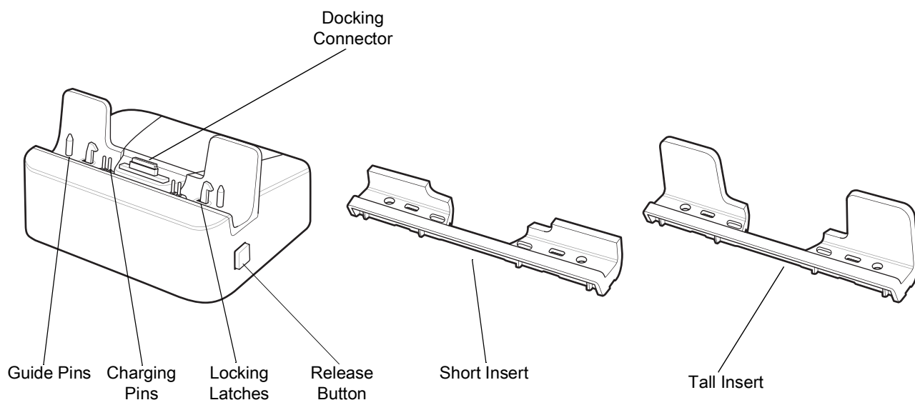
Figure 86 Communication and Charging Cradle - Front View
