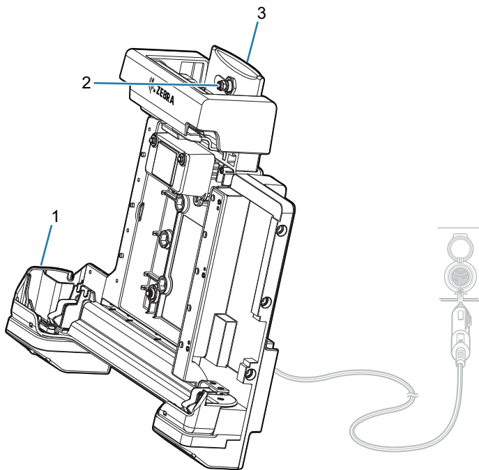
Figure 4 Vehicle Dock Setup
