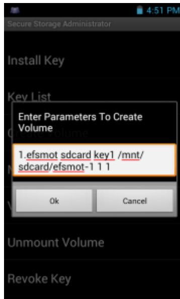
Figure 61: Enter Parameter To Create Volume Dialog Box
