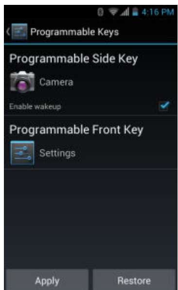
Figure 68: Remapped Button
