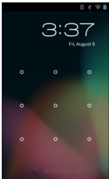
Figure 66: Pattern Screen
