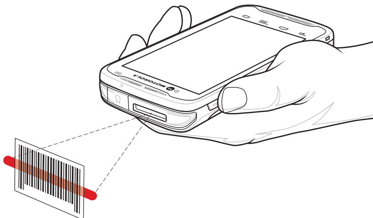
Figure 36: Data Capture
