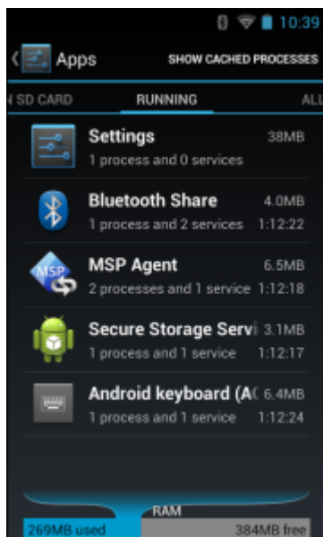
Figure 72: Running Screen
