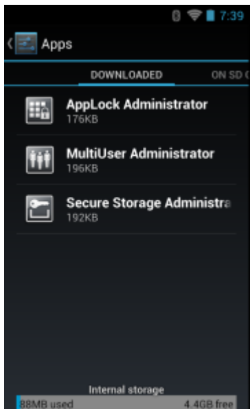
Figure 70: Downloaded Screen
