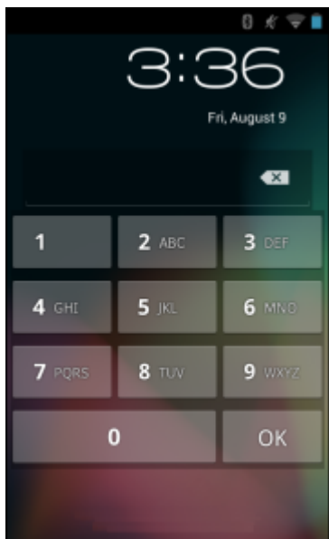
Figure 63: PIN Screen
