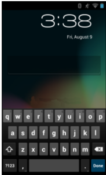
Figure 64: Password Screen
