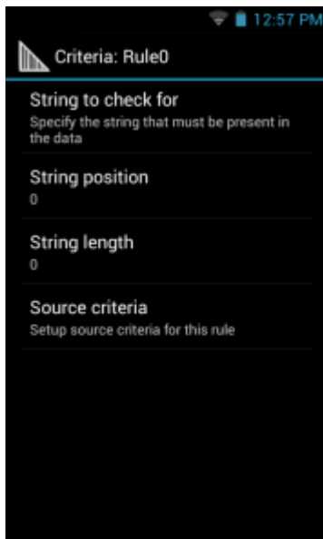
Figure 45: Criteria Screen
