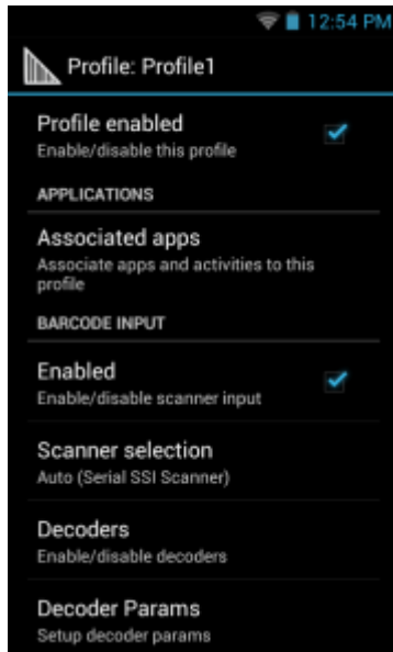
Figure 41: Profile Configuration Screen
