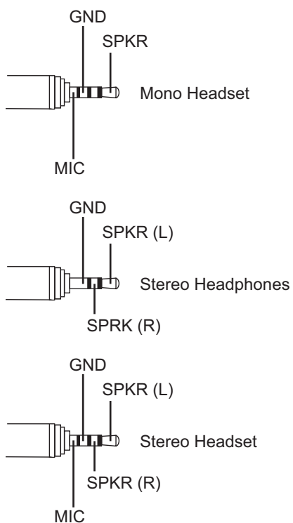
Figure 79: Headset Connector
