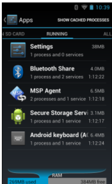
Figure 77: Running Applications
