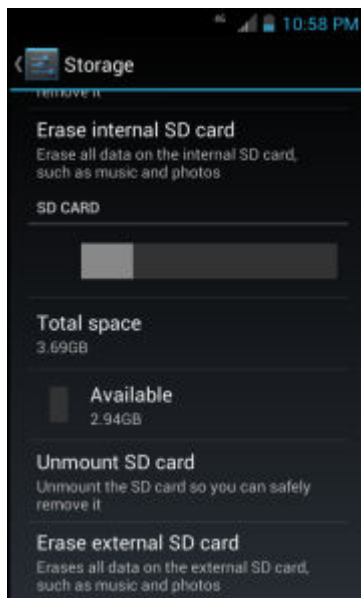
Figure 75: Storage Settings
