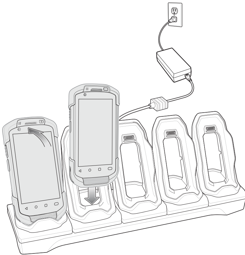
Figure 2-32 TC75x Battery Charging
