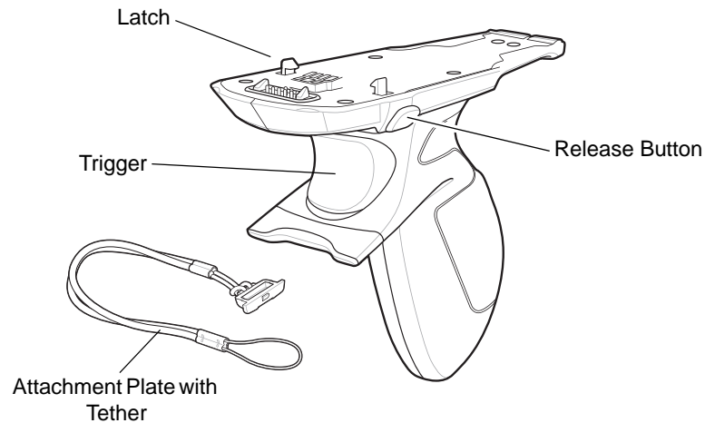
Figure 2-46 Trigger Handle
