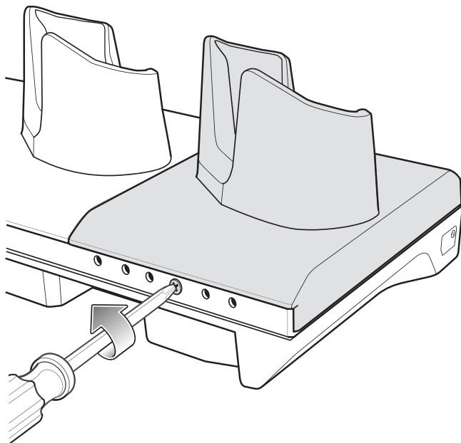
Figure 2-18 Remove Screw
