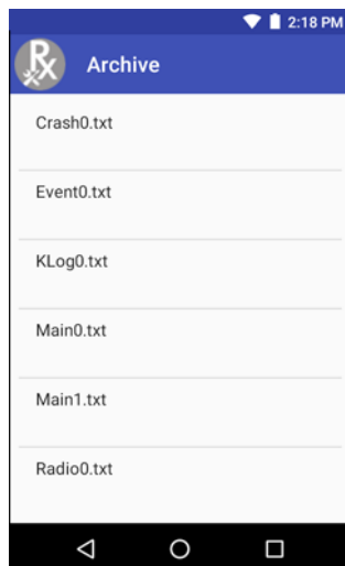
Figure 88 Archive
