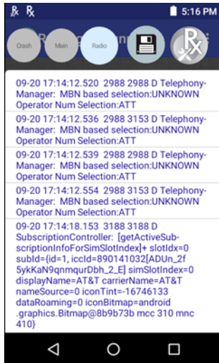
Figure 90 Log File
