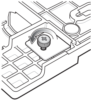
Figure 18 Remove Thumbscrew
