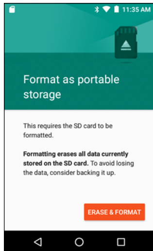
Figure 102 Format Screen
