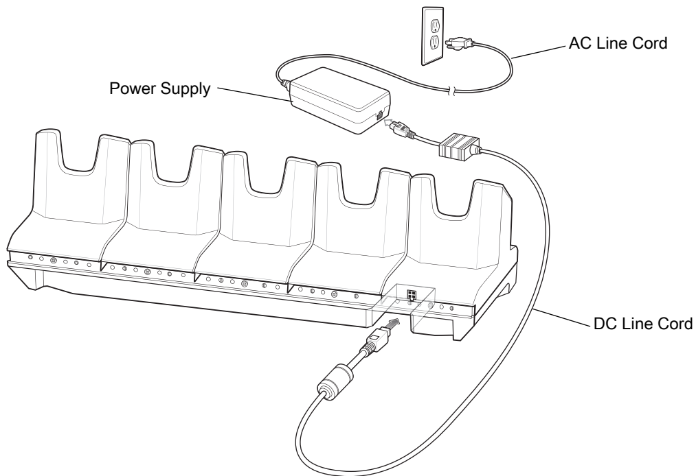
Figure 31 5-Slot Charge Only Cradle Setup
