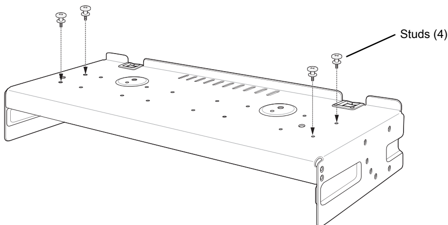
Figure 34 Install Studs
