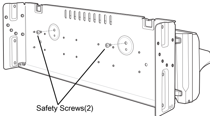
Figure 36 Secure Cradle
