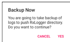
Figure 87 Backup Message
