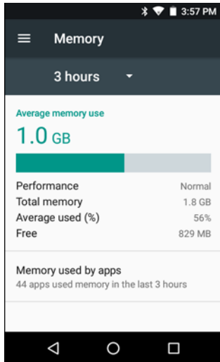
Figure 96 Memory Screen
