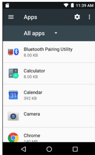
Figure 105 Apps Screen
