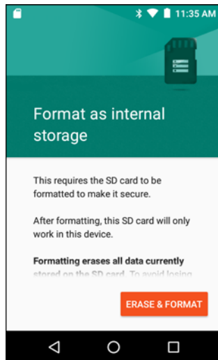
Figure 104 Format Screen
