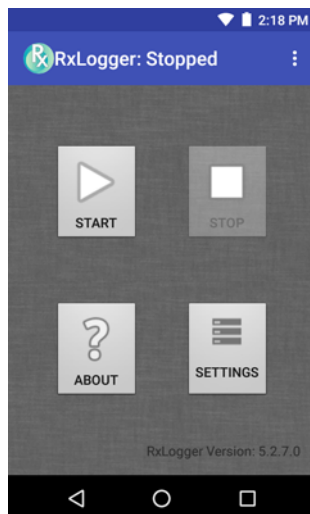
Figure 83 RxLogger
