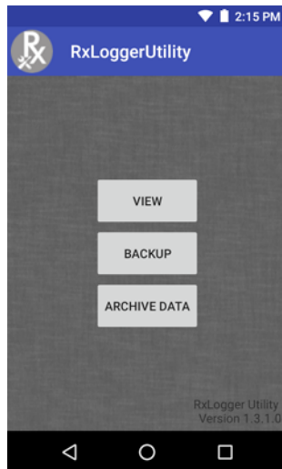
Figure 85 App View
