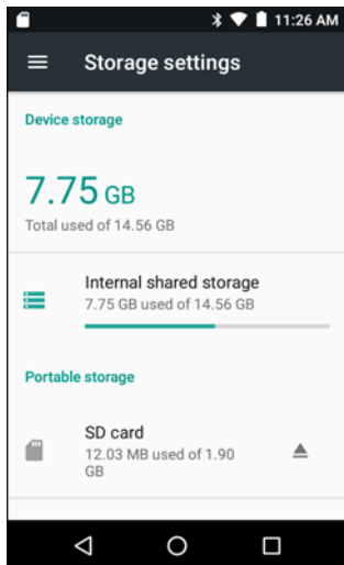
Figure 99 Storage Screen
