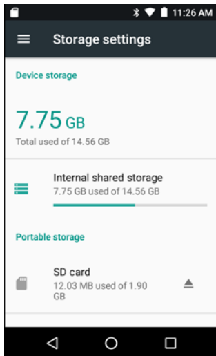
Figure 97 Storage Screen
