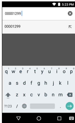
Figure 74 Formatted Data
